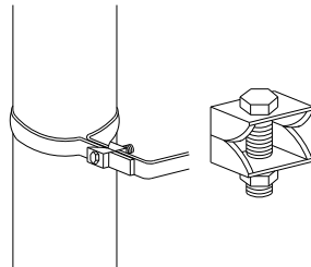
FOR BONDING TAPE TO RAINWATER, PIPES, HANDRAILS & ETC
