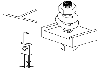
FOR BONDING TAPE TO STEEL STRUCTURES
